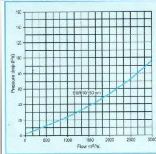
EU 5 TO EU 9 / MERV 5 TO 10
